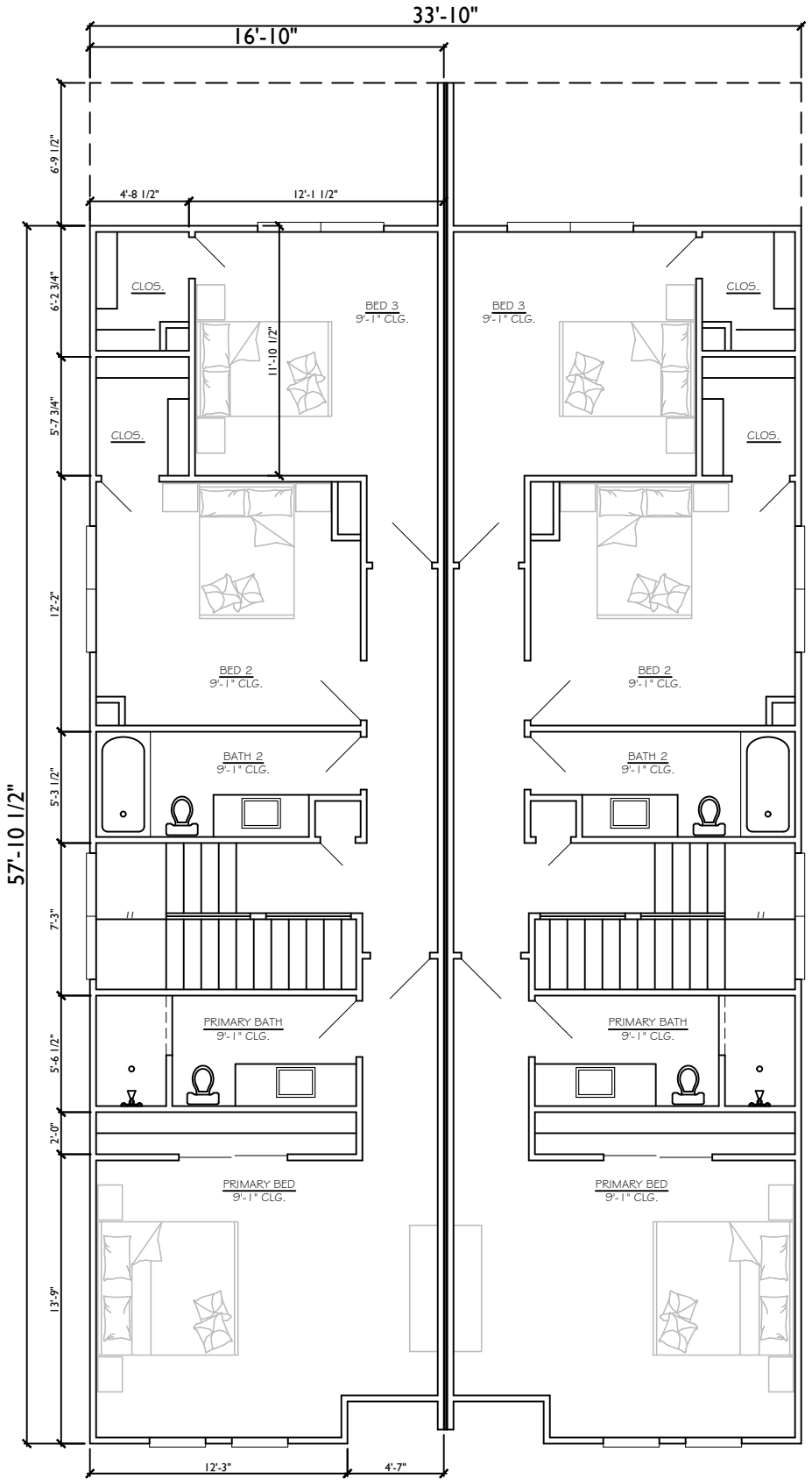
2nd FLOOR Plan No. 1665-1221
