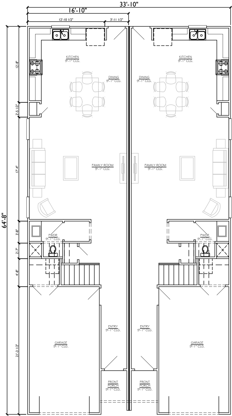
1st FLOOR Plan No. 1665-1221
